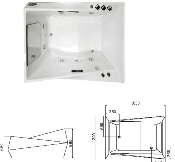
Model: DBB-028 Size: 1800x1300x880mm(650mm)
