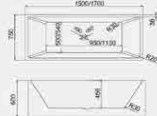
Model: DBB-059 Size: 1500x750x600mm, 1700x750x600mm
