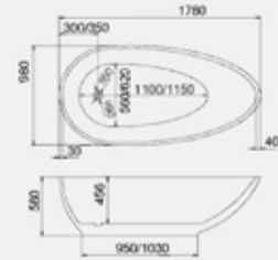
Model: DBB-061 Size: 1780x980x580mm
