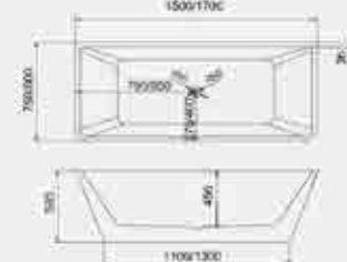
Model: DBB-057 Size: 1500x750x580mm, 1700x800x580mm
