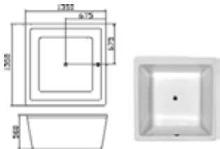
Model: DBB-109 Size: 1350x1350x580mm
