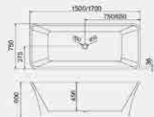
Model: DBB-058 Size: 1500x750x600mm, 1700x750x600mm
