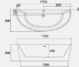
Model: DBB-062 Size: 1700x800x600mm
