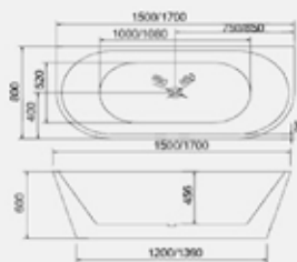
Model: DBB-055 Size: 1500x800x600mm, 1700x800x600mm
